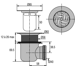
Godet extractible
